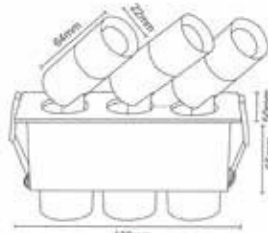
Cutout-40mmx124mm
