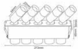
Cutout-40mmx204mm
